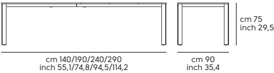
Blade 140/190/240/290x90
