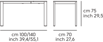
Badù 100/140x70
