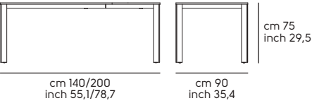
Blade 140/200x90
