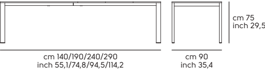
Badù 140/190/240/290x90
